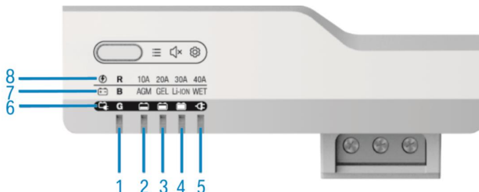
Figure 4-1 BS1225/BS1225-3/BS1240/BS1240-3
