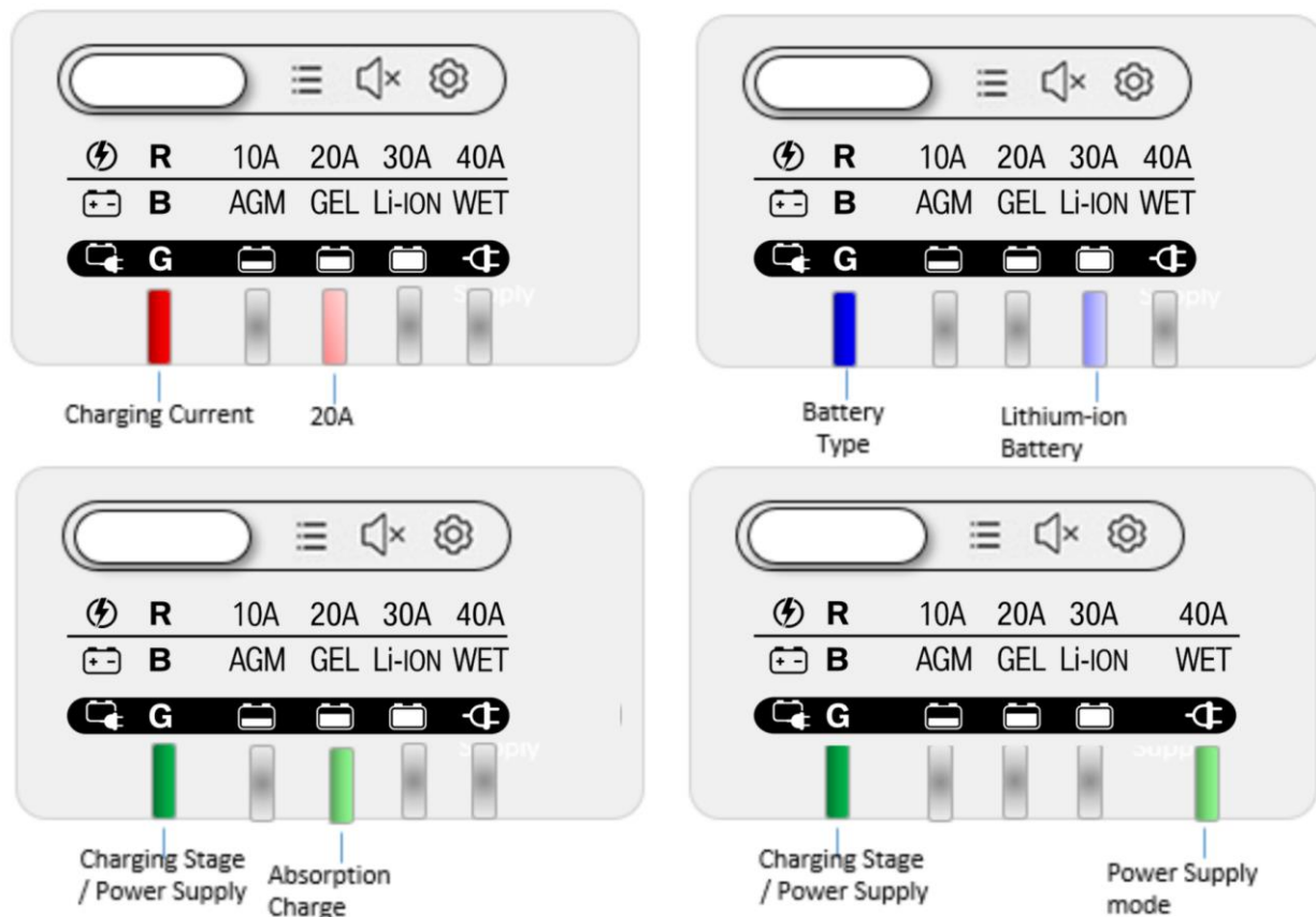
Figure 5-1 BS1225/BS1225-3/BS1240/BS1240-3
