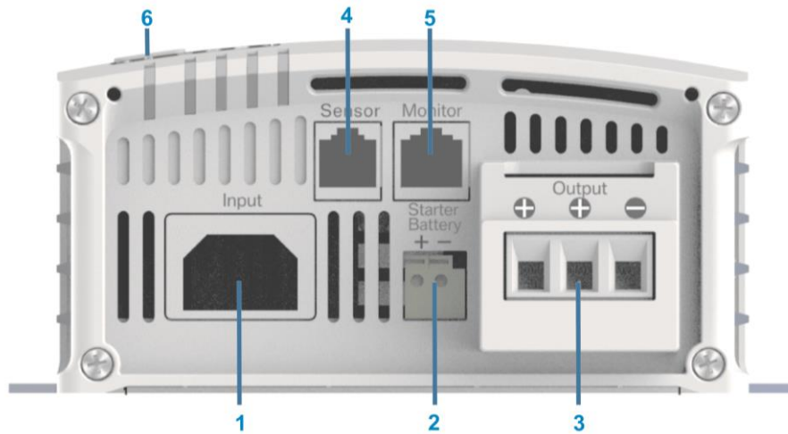
Figure 4-3 BS1225/BS1225-3/BS1240/BS1240-3/ BS2412/BS2412-3/BS2420/BS2420-3
