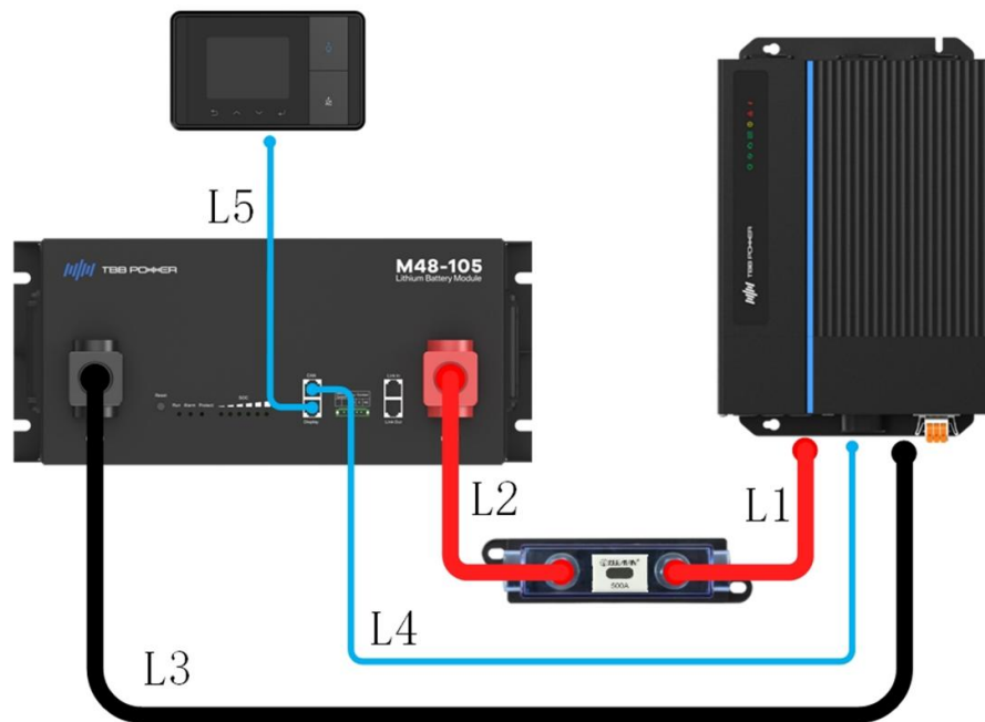
Figure 3-3 Typical wiring diagram
