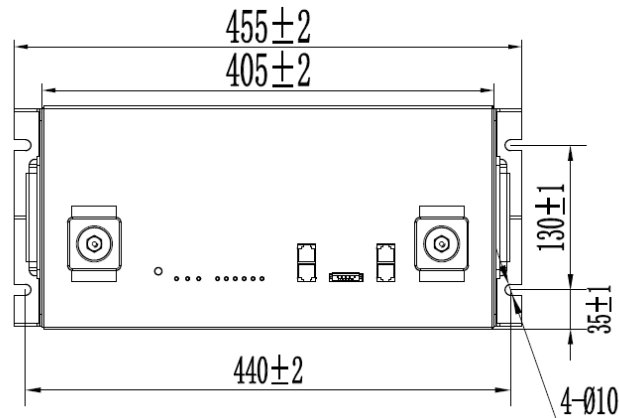
Figure 3-1 Installation positioning requirement
