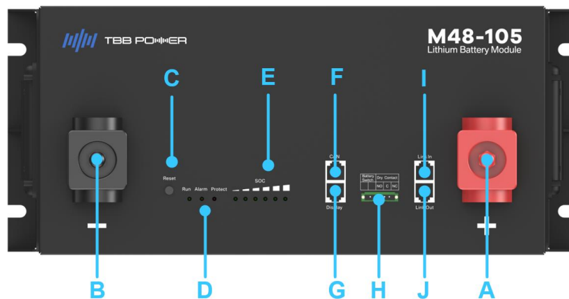
Figure 2-3 M48-105 external interfaces
