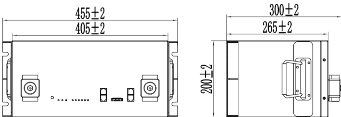
Figure 2-1 Picture of M48-105
