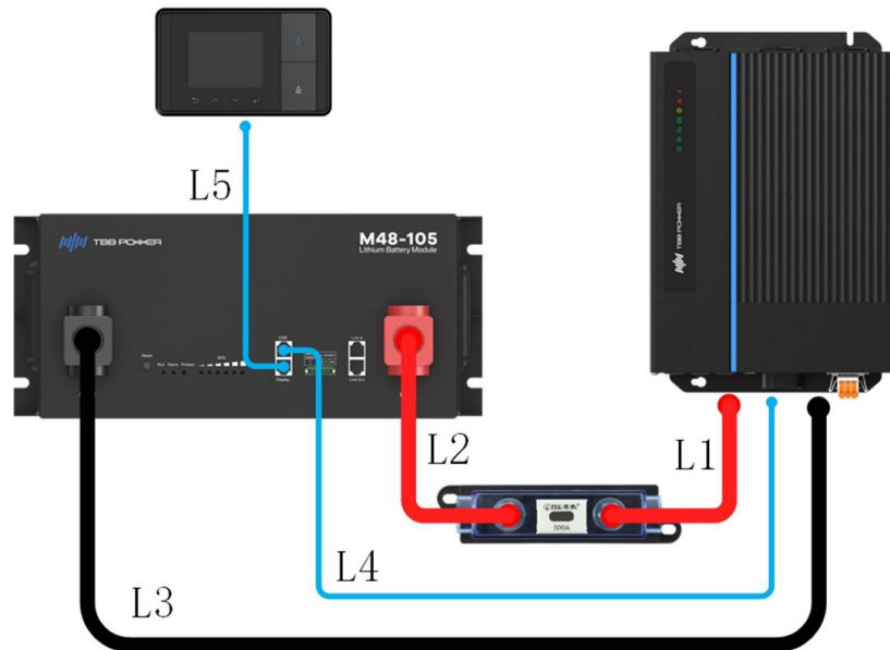
Figure 2-4 Typical wiring diagram (optional VS28-LS)
