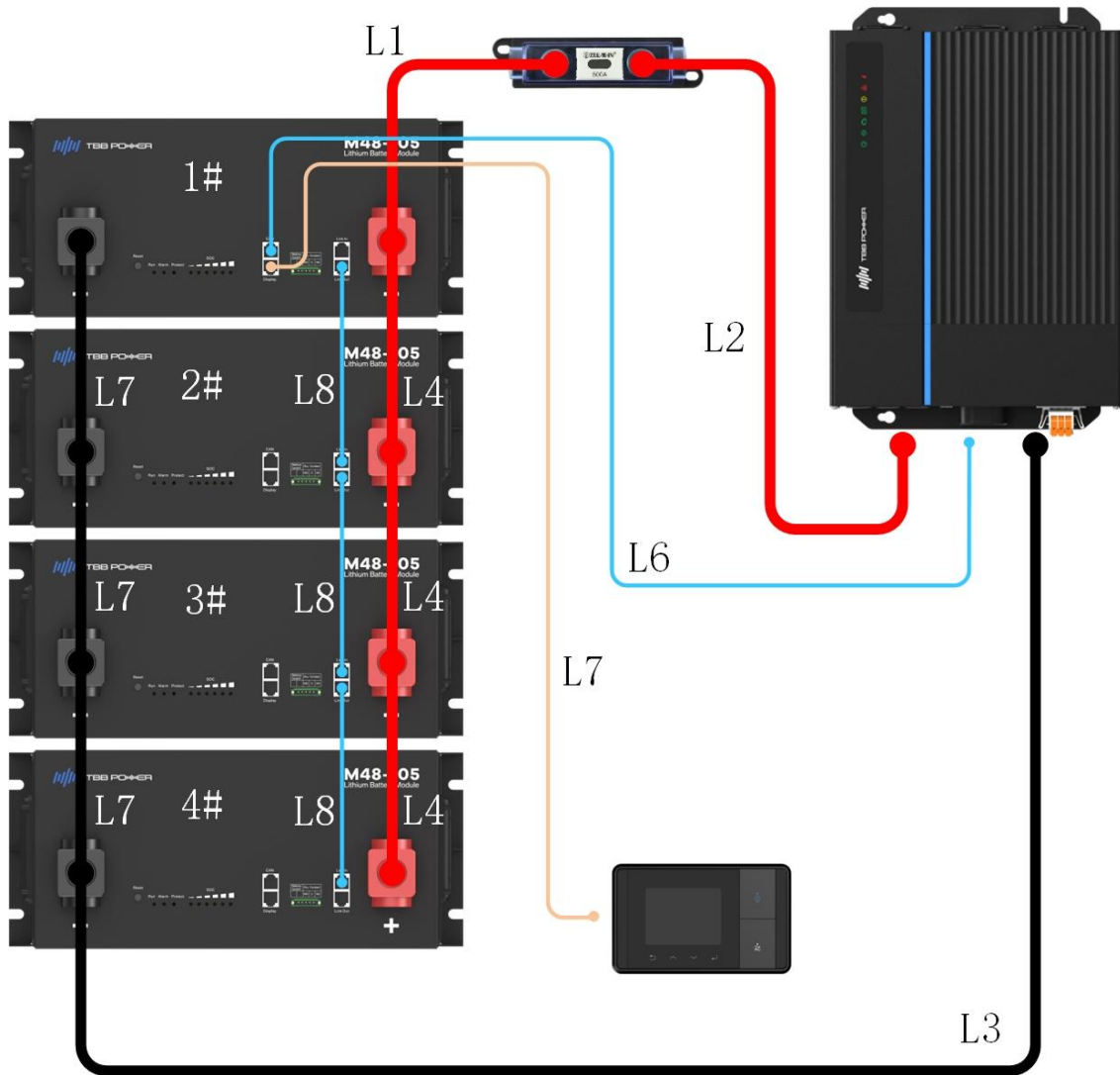
Figure 3-4 Parallel wiring diagram
