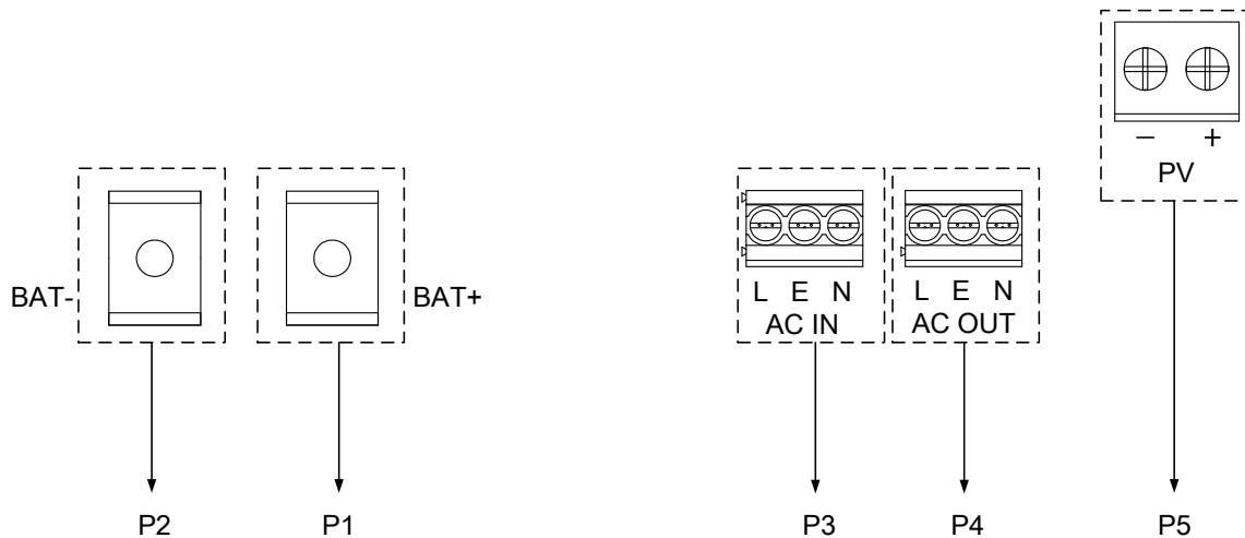
Power Port
